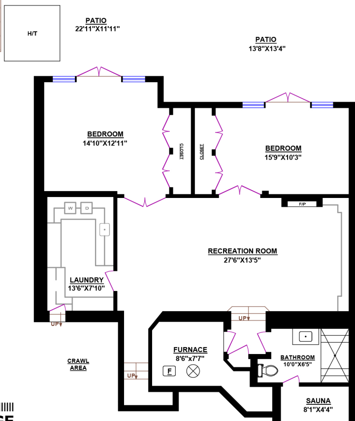
LOWER LEVEL
