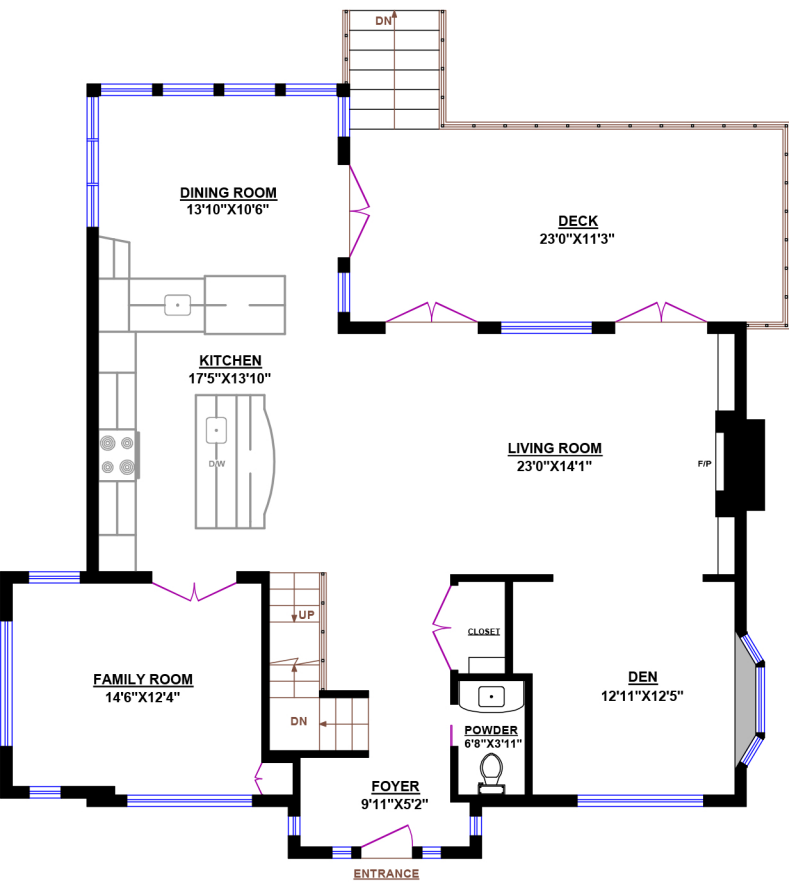
MAIN FLOOR
