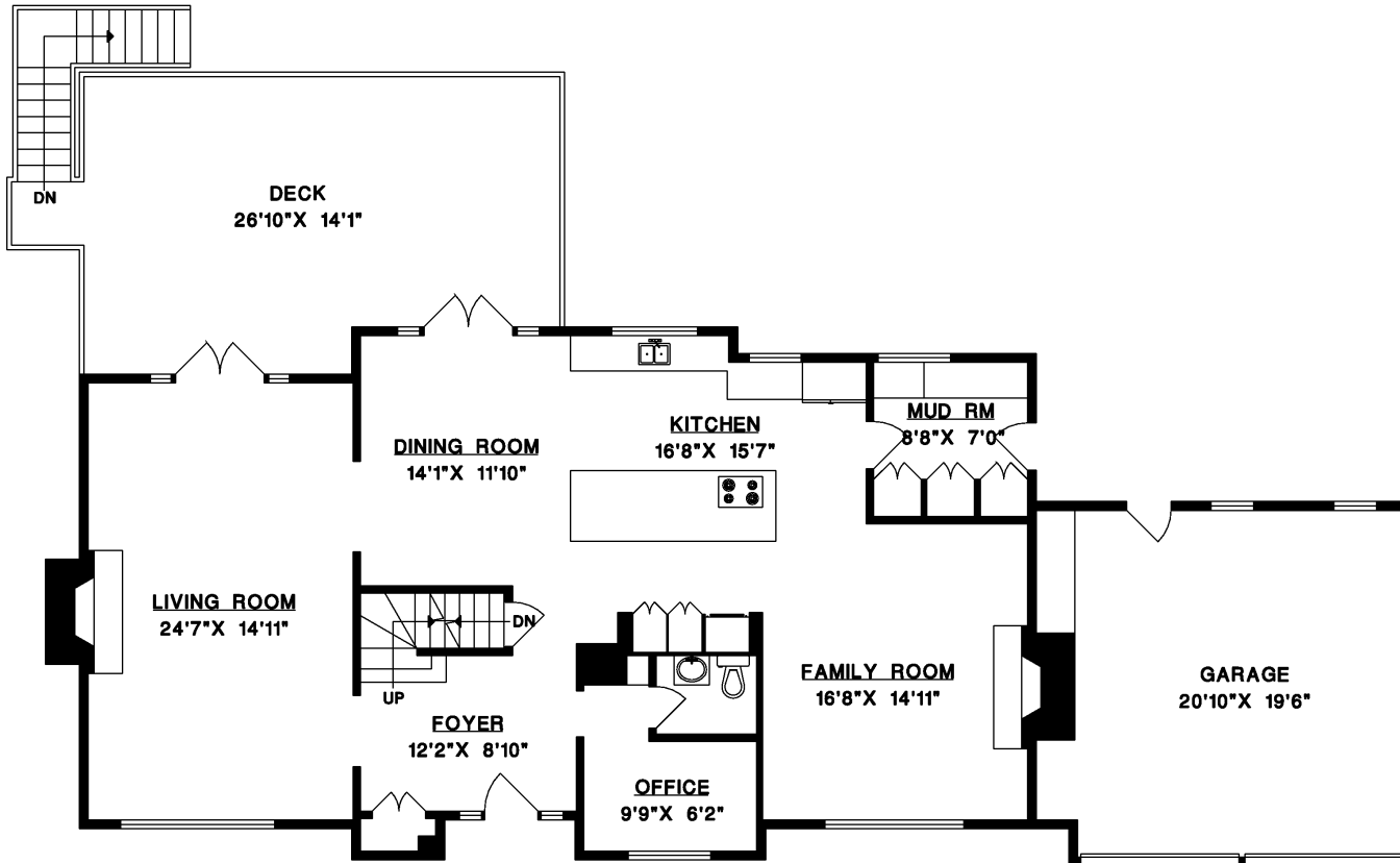
MAIN FLOOR
