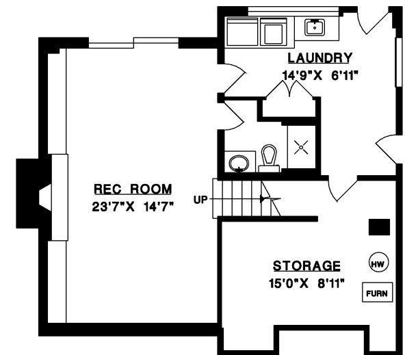
LOWER FLOOR
