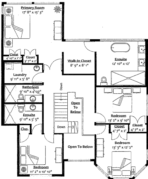
UPPER LEVEL Floor Area: 1,422 Sq. Ft. Ceiling Height: 8'
