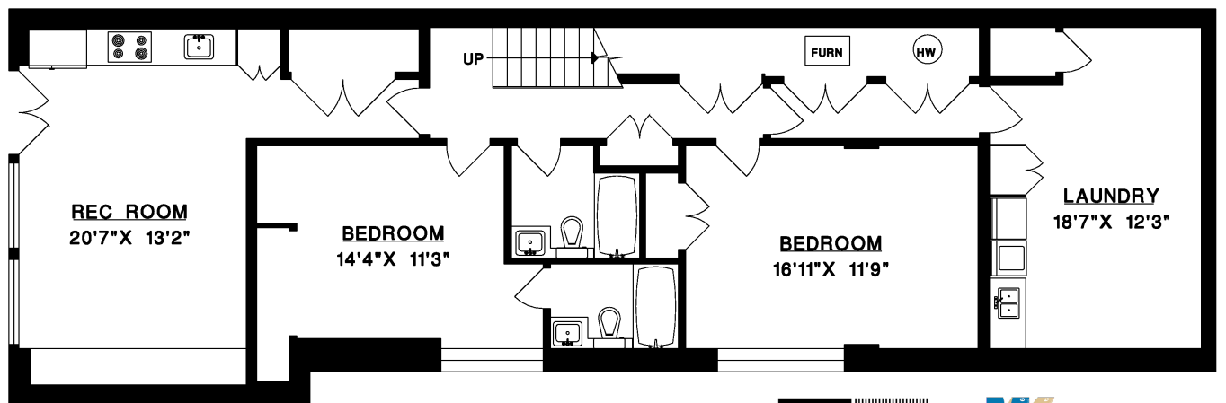
LOWER FLOOR
